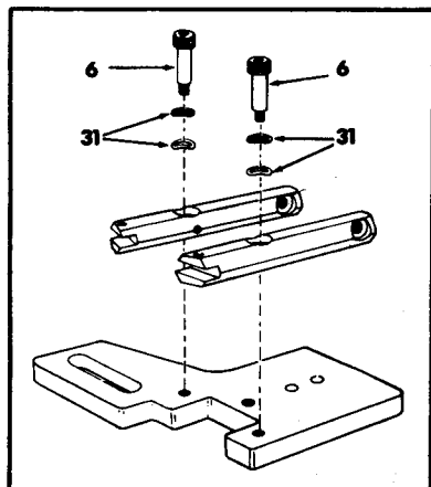
EARLY ROTOR-TRUER DESIGN
